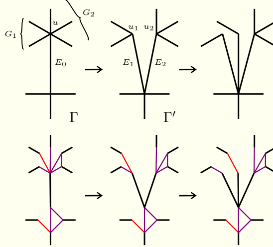
FIGURE 4. Splitting open a cut vertex. In the top row, we have drawn the graph \Gamma . In the bottom row, we draw a ‘blown-up’ view where we insert the local Whitehead graph LW(v, T) at each vertex v , with the purple edges lying in the stable Whitehead graph SW(v, T) and the red edges lying in LW(v, T) but not SW(v, T) .
