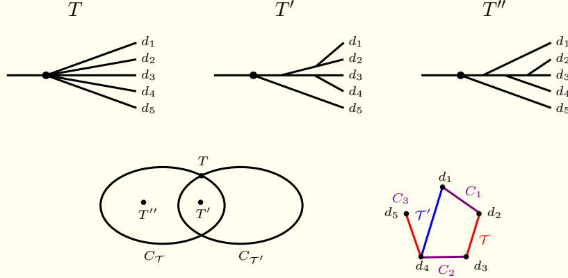
FIGURE 5. An example where T has exactly one gate G of more than one direction and G has exactly 5 directions. The folded train track T' is in C_T \cap C_{T'} . The folded train track T'' is in C_T but not C_{T'} . Bottom right is the graph for determining the relevant inequalities.
