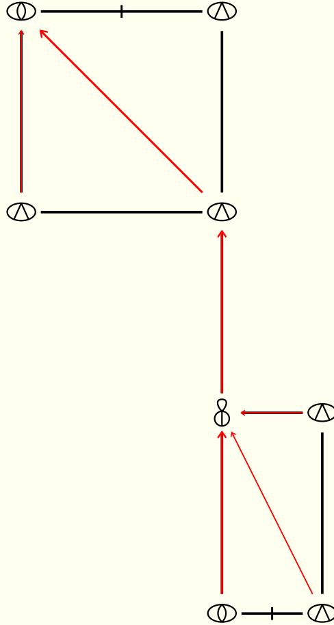
FIGURE 13. The axis bundle of the outer automorphism in Example 5.5.
