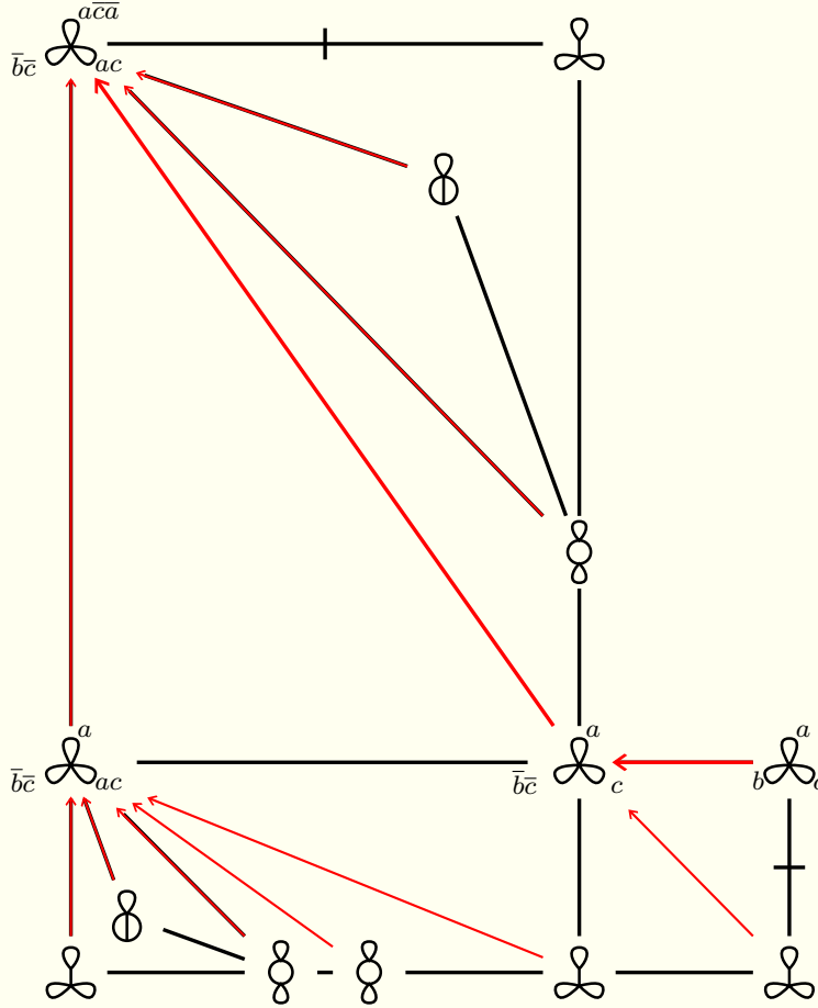
FIGURE 11. The axis bundle of the outer automorphism in Example 5.3.
