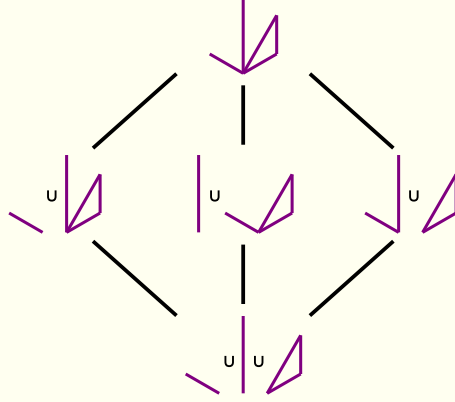
FIGURE 3. The cut decompositions of the top graph, arranged in the partial ordering of fineness.
