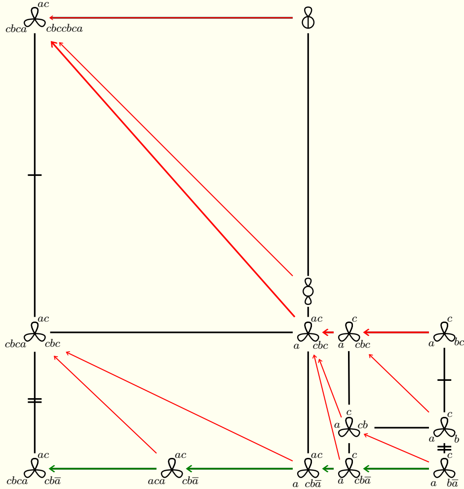
FIGURE 12. The axis bundle and stable axis bundle in Example 5.4.
