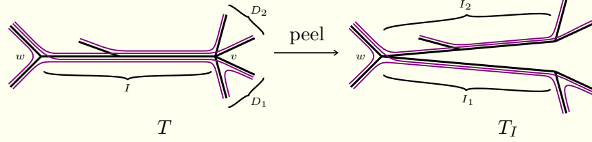
FIGURE 6. Left: A possible peel (D_1, D_2, I) . Right: Peeling off D_1 from D_2 at v along I .
