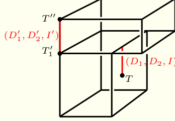
FIGURE 8. B_{T'_1} \cap B_{T''} is a splitting face of B_{T'_1} , so T cannot lie in the interior of a folding face of B_{T'_1} unless B_{T'_1} \cap B_{T''} = B_{T'_1} .
