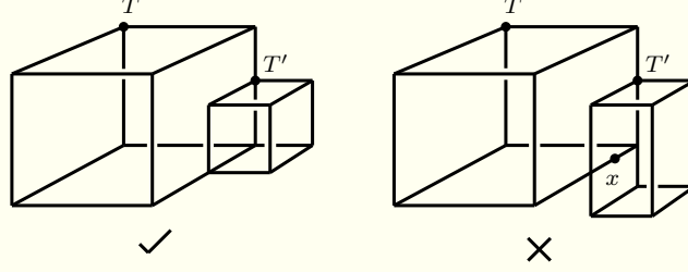
FIGURE 7. If T' be a fully preprincipal train track on a folding face of B_T , then B_T \cap B_{T'} is a splitting face of B_{T'} , as in the left, and not on the right.
