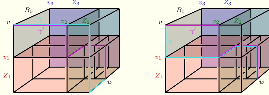
FIGURE 9. For Lemma 4.6, we first argue the case when the initial edges of \gamma and \gamma' agree (left), we then argue one case when the initial edges of \gamma and \gamma' differ (right).
